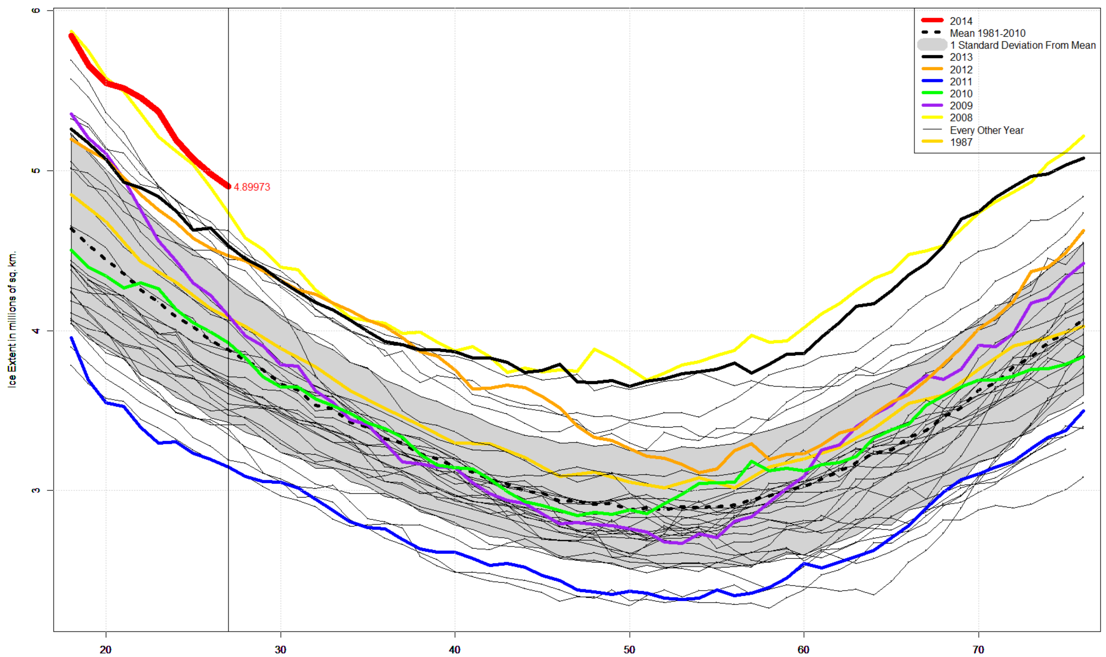
Antarctic Sea Ice Extent Day 27 1978 to 2014
